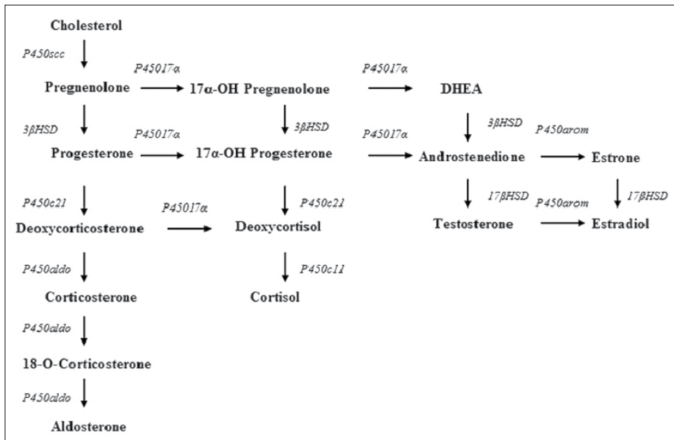
Figure 1. Biochemical pathway for steroid hormone synthesis (Manca, 2008)
